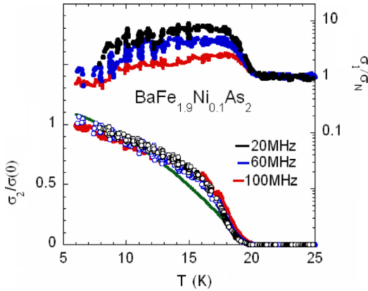
Fig. 4. (Color online) Temperature dependence of the real \sigma_1/\sigma_N (filled symbols) and imaginary \sigma_2/\sigma_2(0) (open symbols) parts of the conductivity normalized to the value \sigma_N at 25 K for the optimally doped \text{BaFe}_{1.9}\text{Ni}_{0.1}\text{As}_2 crystals. Solid line is calculated with 1 - (T/20)^2 .
