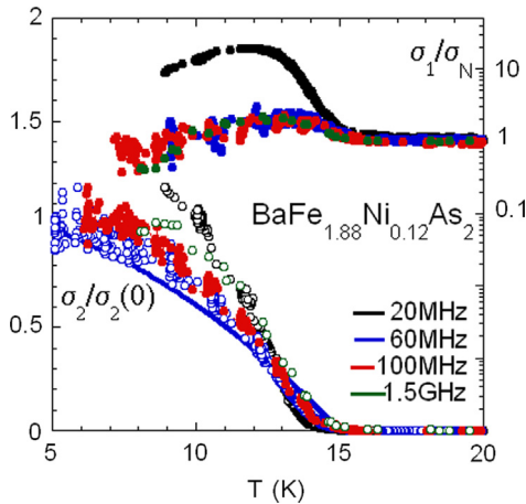
Fig. 5. (Color online) Temperature dependence of the real \sigma_1/\sigma_N (filled symbols) and imaginary \sigma_2/\sigma_2(0) (open symbols) parts of the conductivity normalized to the value \sigma_N at 25 K for the over doped \text{BaFe}_{1.88}\text{Ni}_{0.12}\text{As}_2 crystals. Solid line is calculated with 1 - (T/16)^2 .
