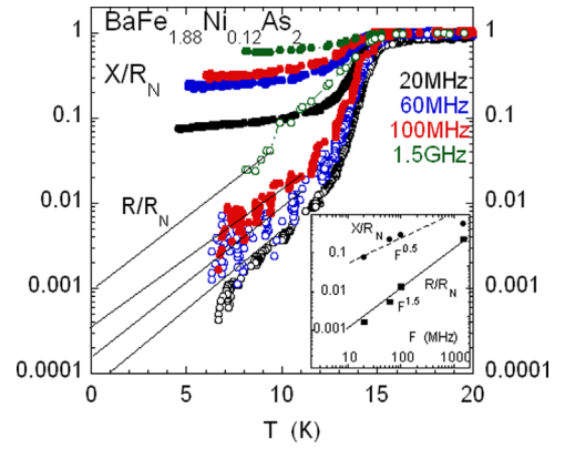
Fig. 2. (Color online) Temperature dependence of X/R_N (filled symbols) and R/R_N (open symbols) of surface impedance normalized to the value R_N obtained at 25 K for the overdoped \text{BaFe}_{1.88}\text{Ni}_{0.12}\text{As}_2 crystals. Inset: Frequency dependences of X/R_N and R/R_N at 10 K.
