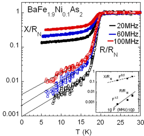
Fig. 1. (Color online) Temperature dependence of X/R_N (filled symbols) and R/R_N (open symbols) of surface impedance normalized to the value R_N obtained at 25 K for the optimally doped \text{BaFe}_{1.9}\text{Ni}_{0.1}\text{As}_2 crystals. Inset: Frequency dependences of X/R_N and R/R_N at 10 K.
