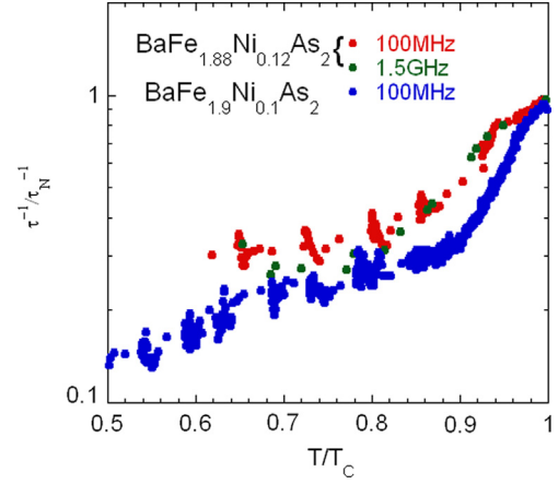
Fig. 6. (Color online) The temperature dependence of the quasiparticle scattering rate deduced from the conductivity \sigma_1/\sigma_N with Eq. (6).
