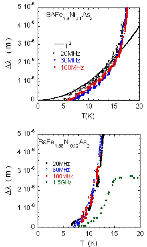
Fig. 3. (Color online) Temperature dependence of the London penetration depth variation \Delta\lambda = \lambda - \lambda(0) at different frequencies.
